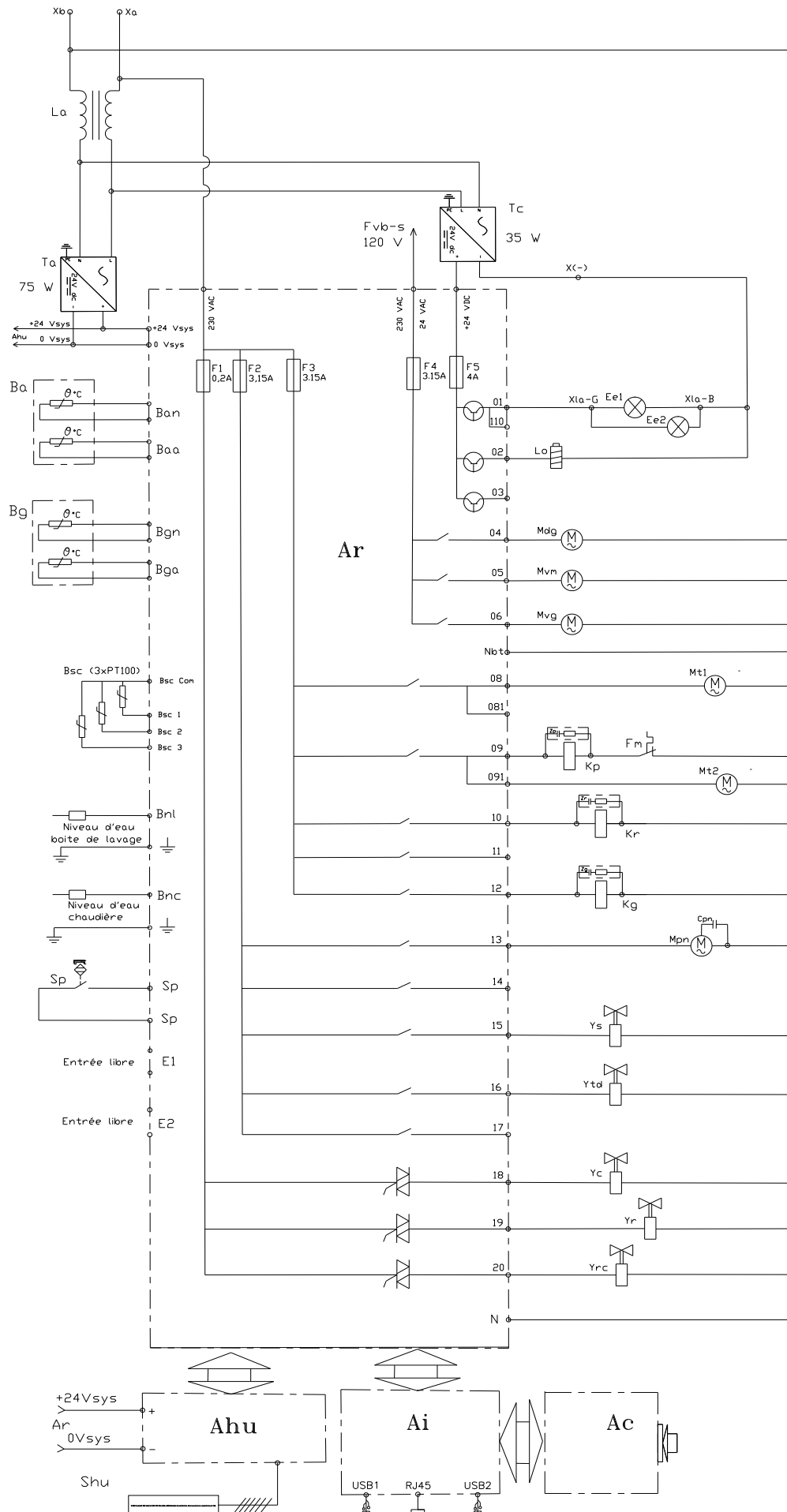
Wiring diagram
