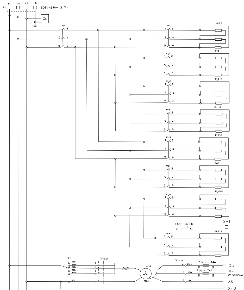
Power diagram 10GN2/1 – 208V-240V
