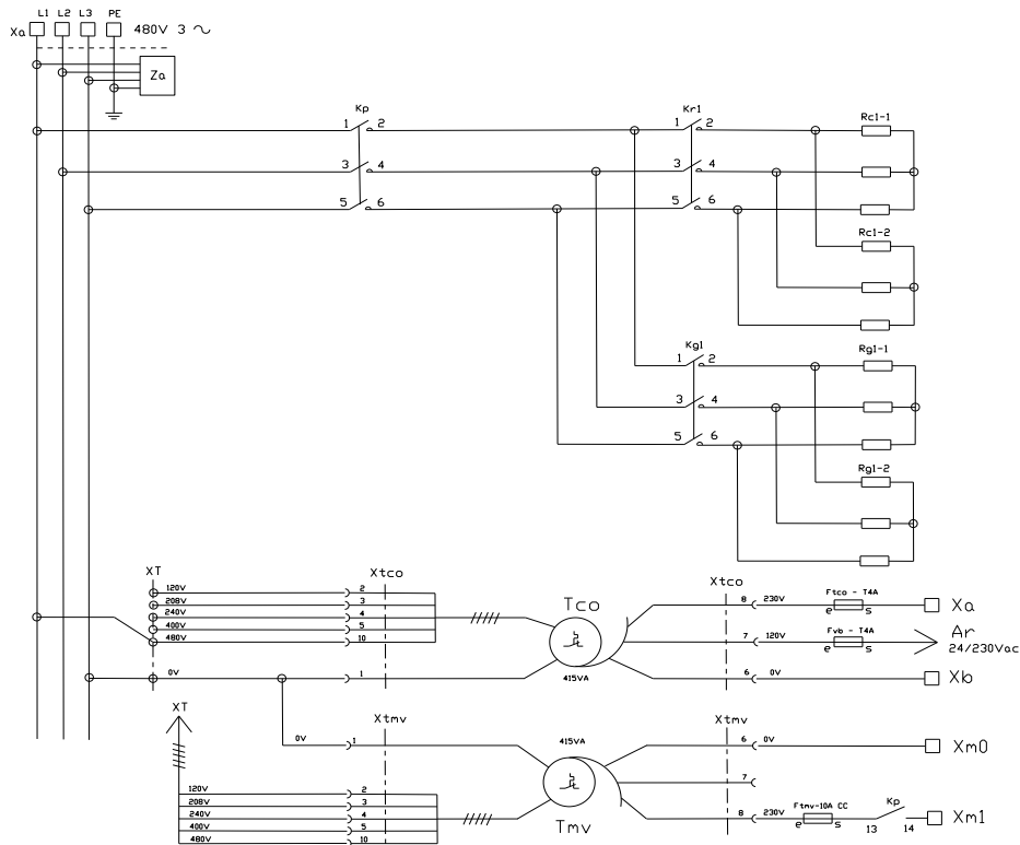
Power diagram 10GN2/1 – 208V-240V
